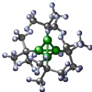
Fig. 15 Tetra- tert -butyltetraboratetrahedrane
