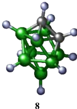
Fig. 8 Closo -1,2- \text{C}_2\text{B}_8\text{H}_{10}
