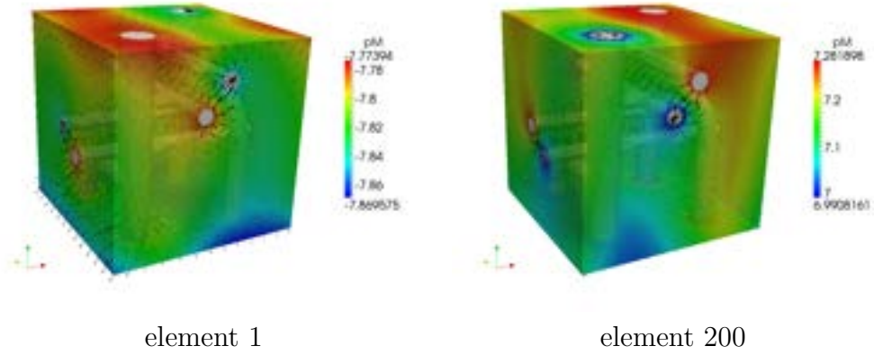
Figure 15: Perfusion reconstruction at the microscopic level — pressure p_M(x', \cdot) and perfusion velocities w_M(x', \cdot) in matrix, as evaluated at two different macroscopic points (elements).
